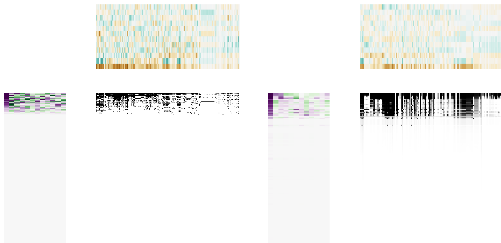
Figure 3 Visual representation of the left (green/purple; left-side matrix) and right (green/brown; top matrix) subspaces, alongside the adjacency matrix of the food web they encode (greyscale). Where the color saturation is the magnitude of the latent trait value. The European metaweb is on the left, and the imputed Canadian metaweb (before data inflation) on the right. This figure illustrates how much structure the left subspace captures. As we show in fig. 6, the species with a value of 0 in the left subspace are species without any prey.
